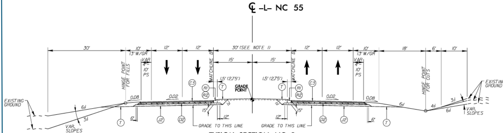
TYPICAL SECTION NO. 2
