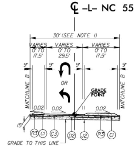
TYPICAL SECTION NO. 2A
